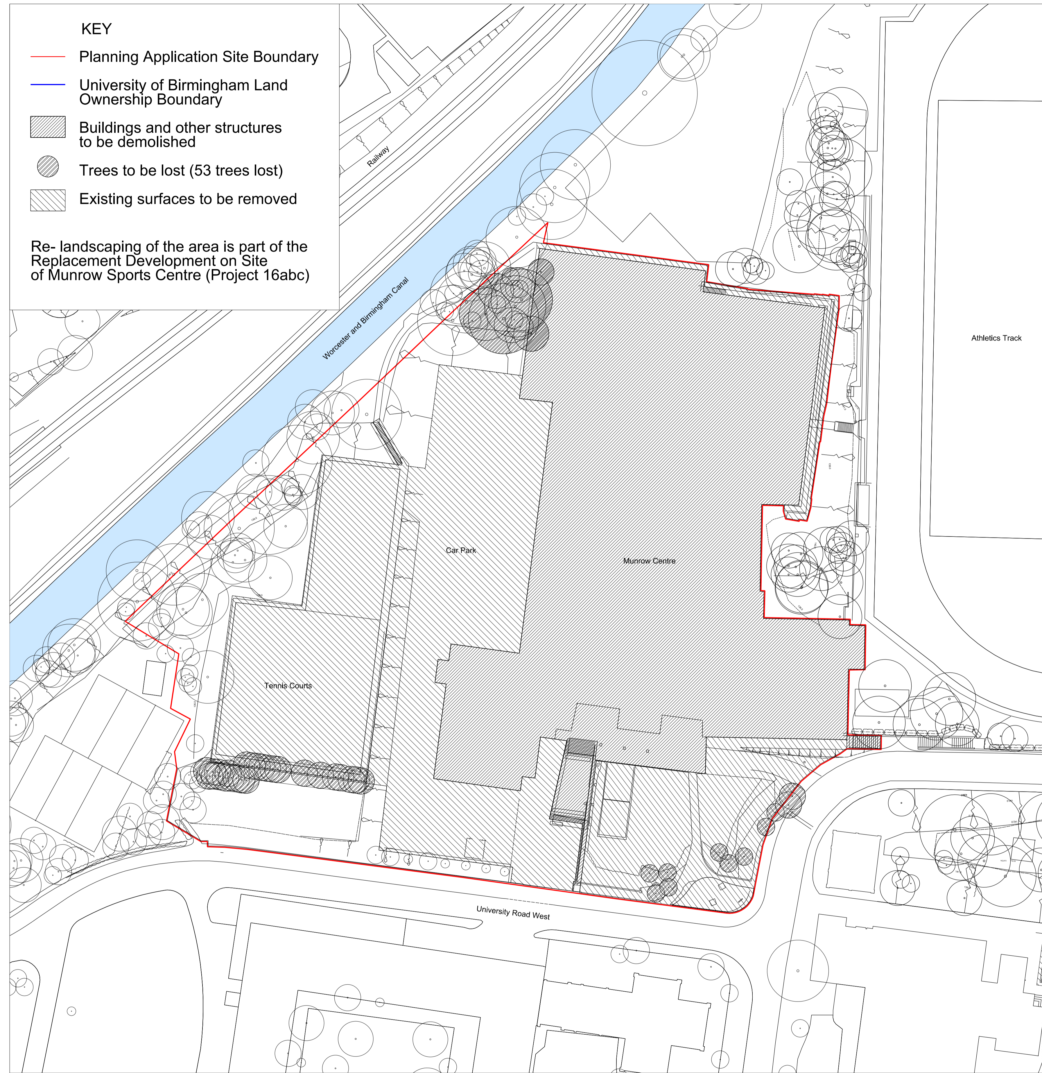
Project 14: Demolitions Block Plan - scale 1:500
