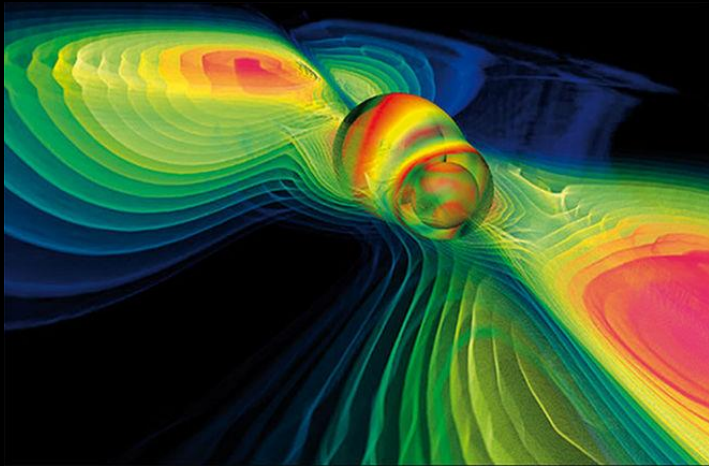
Observation of Gravitational waves
